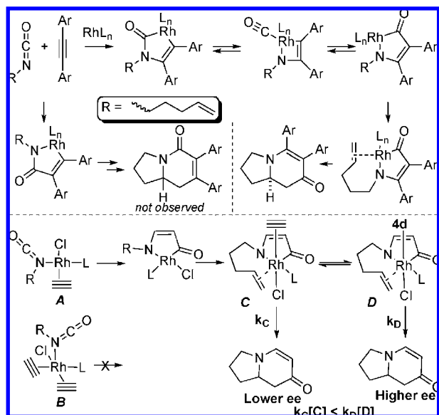
Figure 7. Proposed mechanism and role of the additive.
