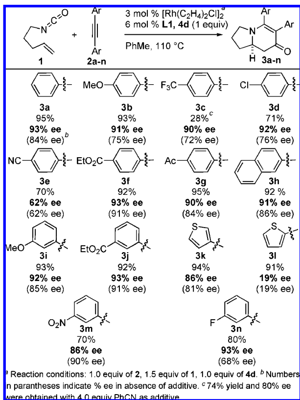
Figure 5. Tolane substrate scope in presence of additive.
